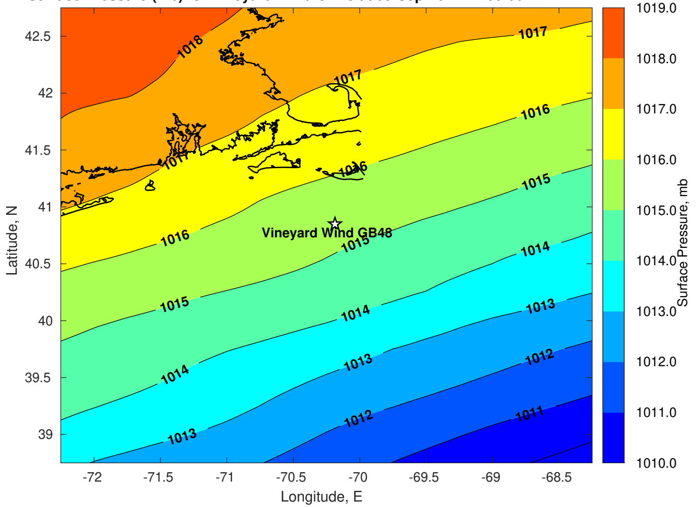
Surface Pressure (mb) for Vineyard Wind GB48 at 09-Sep-2022 12:00:00
