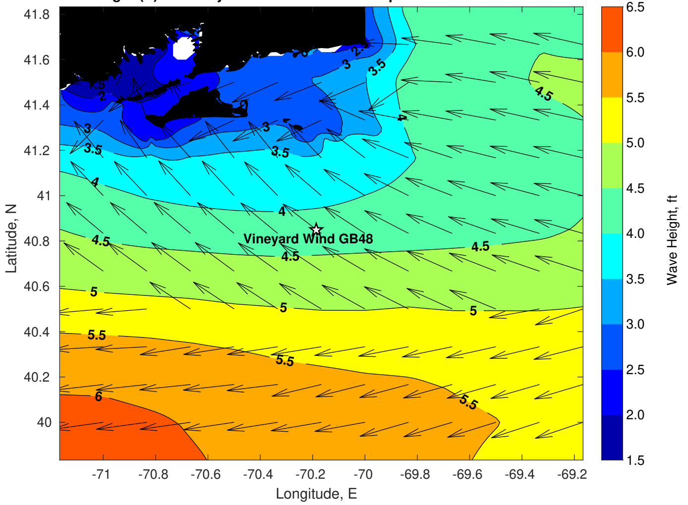
Wave Height (ft) for Vineyard Wind GB48 at 07-Sep-2022 12:00:00
